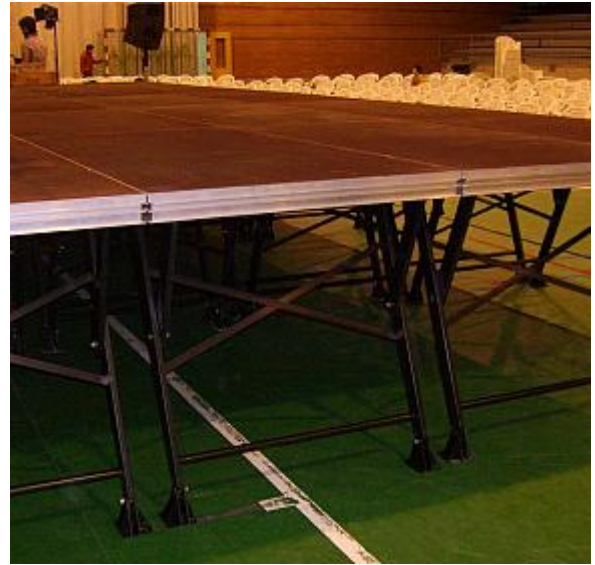
Scissor pallets
